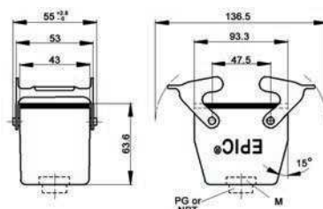
standard profile
