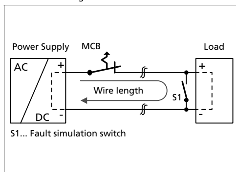
Fig. 24-5 Test circuit
