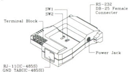
Figure 1-1 External View
