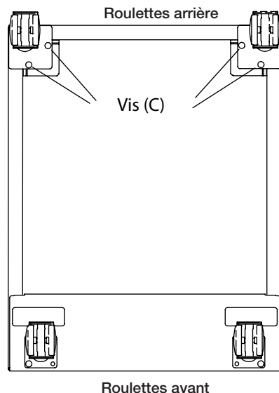
FIGURE 3 : Assemblage complet.
