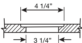
Drain Details: (U.S.)
