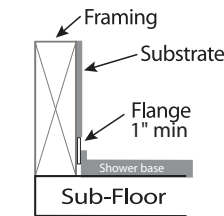
Flange Details: (U.S.)
