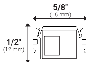
Fixture Cross-Section
