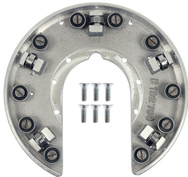
Rear Plate Complete -J2 p/n 03094
