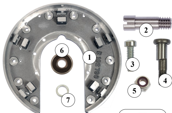
ITEM# 03094 REAR PLATE COMPLETE USED IN: SPACER & PLATES THIS KIT CONSISTS OF:
