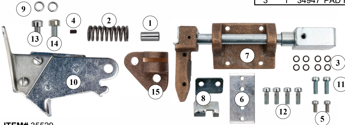
ITEM# 35529 STRAND LOCK/PIVOT PLATE Kit - J LASHER USED IN: J DRIVE HOUSING ONLY THIS KIT CONSISTS OF:
