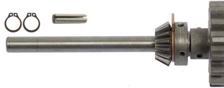
R.H. / L.H. Pinion Assy Kit - J2 p/n 35481
