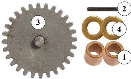
ITEM# 33274 IDLER GEAR AND SHAFT KIT
