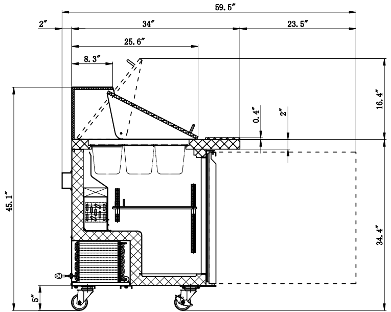
SECTION VIEW
