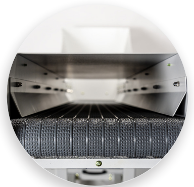
21.5" wide rubber conveyor belt removes shredded waste.
