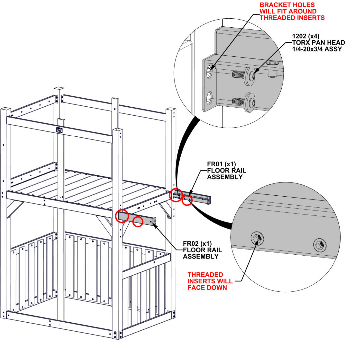
FR02 FLOOR RAIL ASSEMBLY - A4M05937 (x1) 18 1/4"X3 1/8"X1 15/16" (50x80x429)
