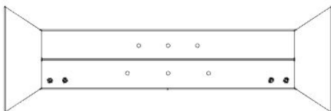
S11 STRINGER ASSEMBLY - A4M05696 (x2) 60 11/16"x3 1/8"x13/16" (20x80x1542)
