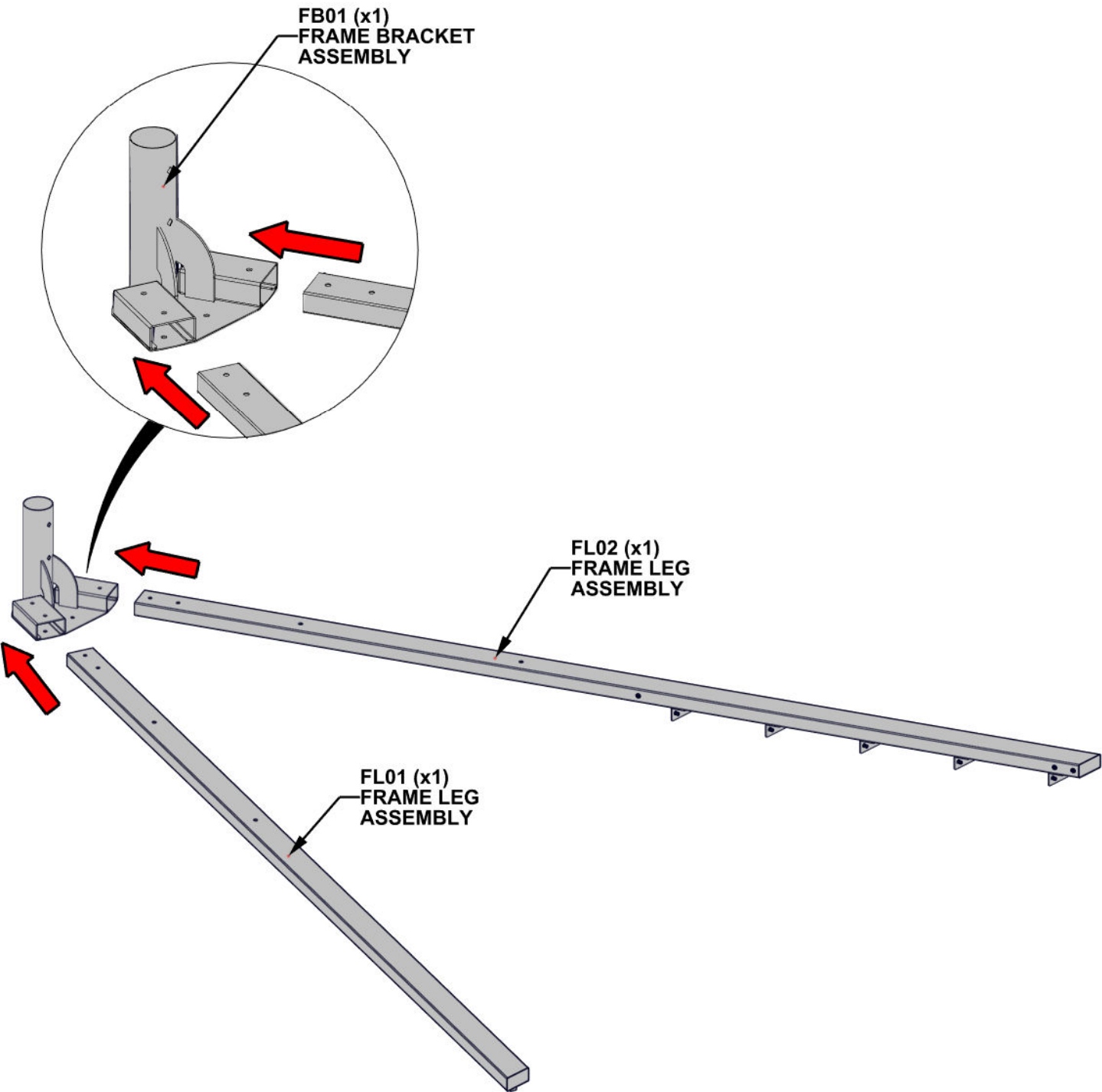
FB01 FRAME BRACKET ASSEMBLY - A4M06615 (x1) 12 3/4"x8 7/8"x13 7/8" (352x227x324)
