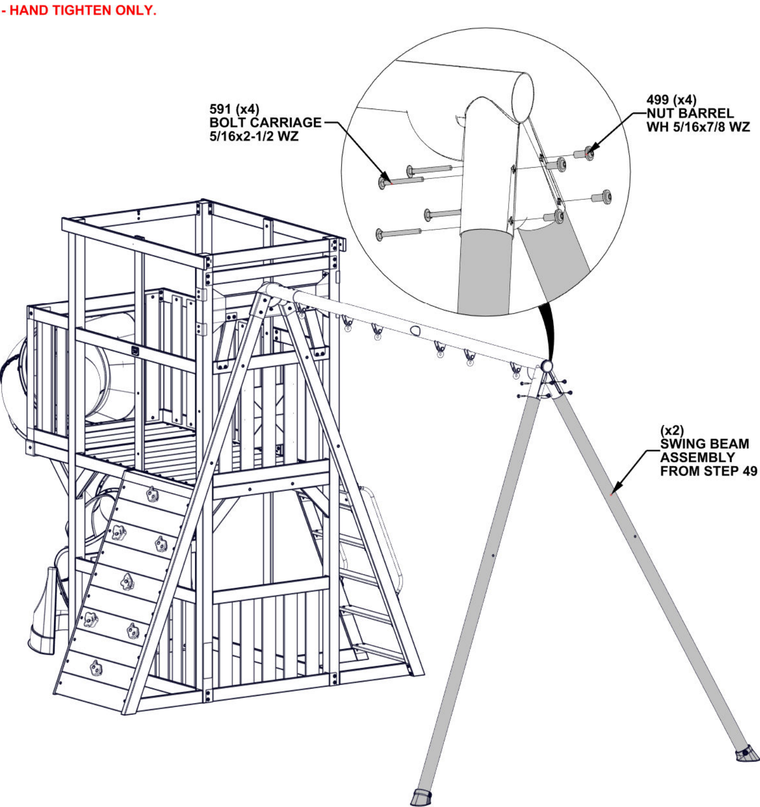
SWING BEAM ASSEMBLY FROM STEP 49 (x2)
