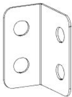
6821 BRACKET - A4M06821 (x2) 3 3/8"x2 1/2"x1 3/4" (65x45x87)
