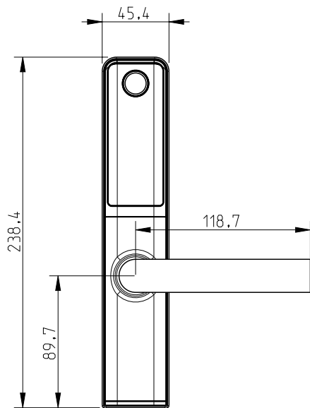
External lock body
