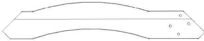
C01 CORBEAU - W2A03198-1 (x2) 1 7/16"x3 3/8"x35 1/8" (36x86x893)
