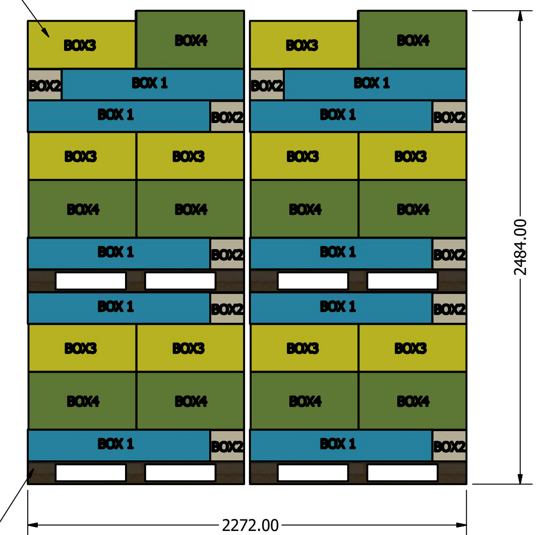
End view
