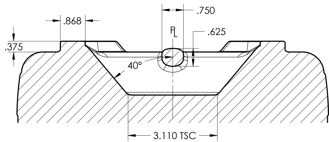
SECTION B-B
