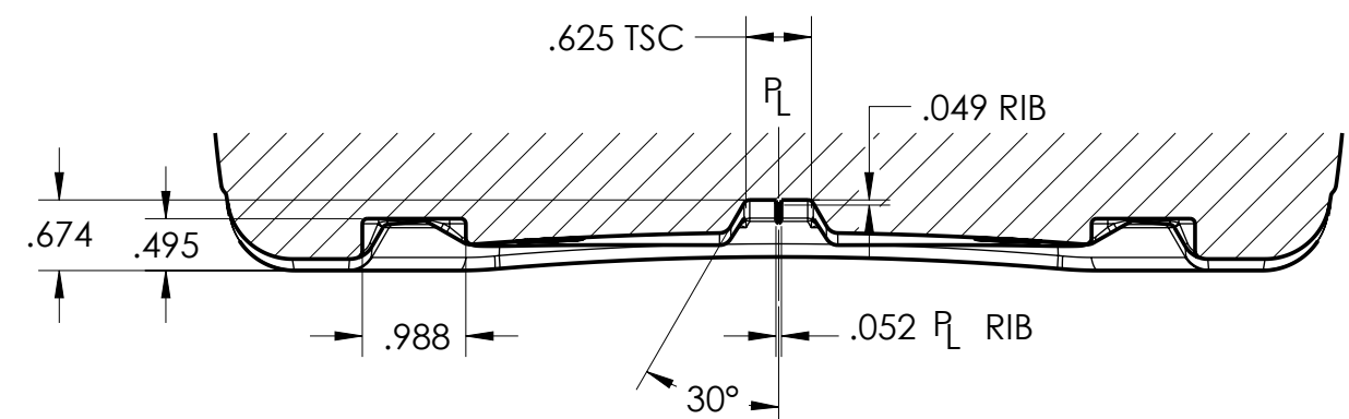
SECTION C-C
