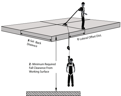
Figure 11 - MRFC Non-Overhead Anchorage
