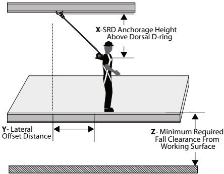
Figure 10 - MRFC Overhead Anchorage
