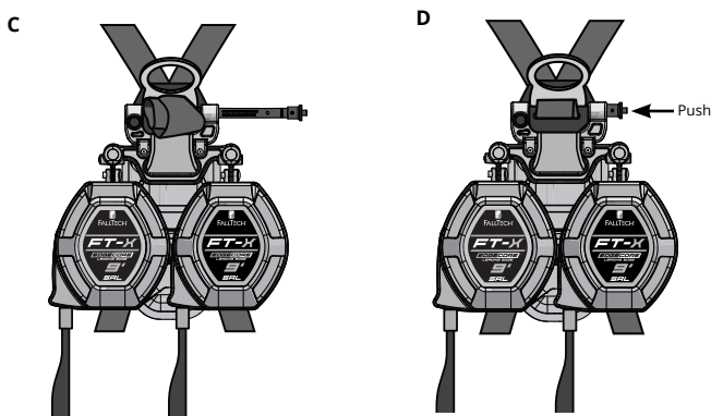
Figure 6 - FT-X® EdgeCore Arc Flash Tie-Back Class 2 Leading Edge SRL-P Installation (continued)
