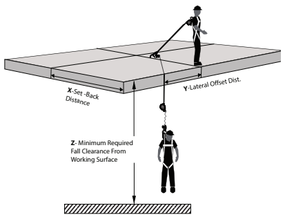
Figure 14 - MRFC Non-Overhead Anchorage
