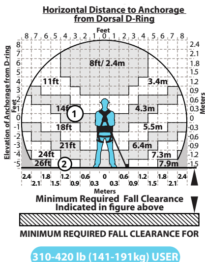
Figure 15 - FT-X Minimum Required Fall Clearance for 310 to 420 lbs. (141 to 191 kg) Users
