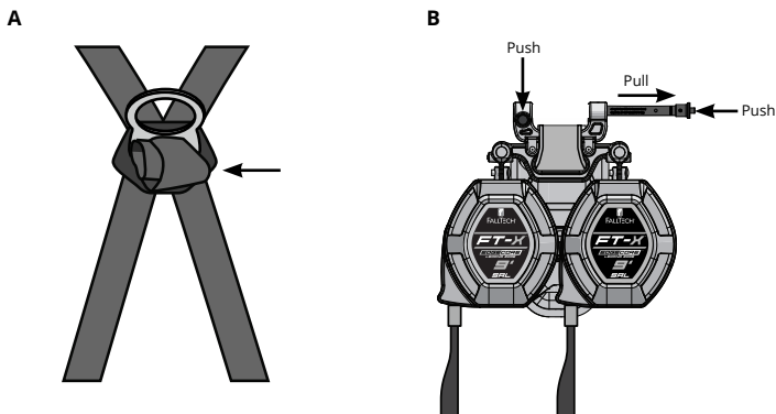
Figure 6 - FT-X® EdgeCore Arc Flash Tie-Back Class 2 Leading Edge SRL-P Installation
