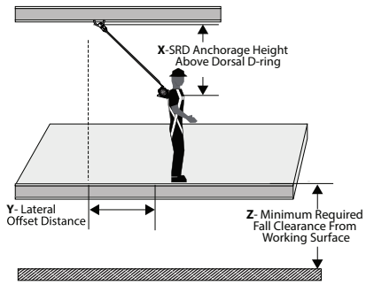
Figure 13 - MRFC Overhead Anchorage
