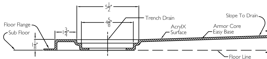
CROSS SECTION OF SHOWER BASE
