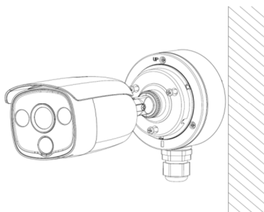
Figure 7, Combine the Junction Box's Cover with its Body
