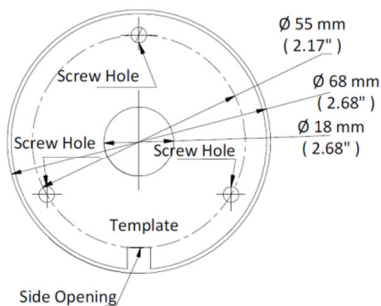
Figure 2, Drill Template
