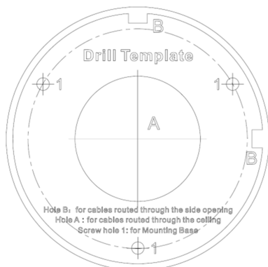
Figure 5, Drill Template
