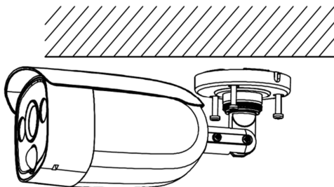
Figure 4, 3-Axis Adjustment
