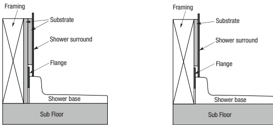
Flange Details: Fire Rated Walls (U.S.) Flange Details: (U.S.)
