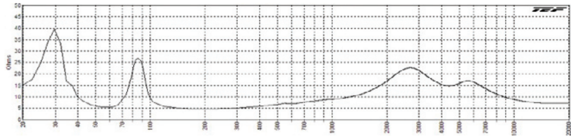
PM8CX Impedance
