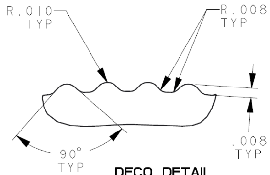
DECO DETAIL SCALE 12:1
