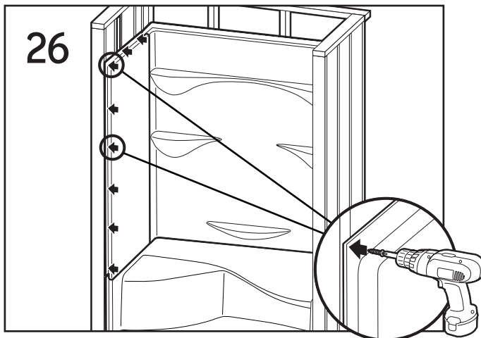
Fasten flanges along top of left side wall with fasteners of choice (see Pre-Installation Planning #12) into each corresponding stud. Fasten side (vertical) flanges to side studs 8" (200mm) on center.
