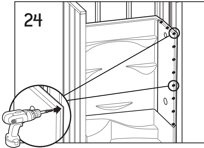
Fasten flanges along top of right side wall with fasteners of choice (see Pre-Installation Planning #12) into each corresponding stud. Fasten side (vertical) flanges to side studs 8" (200mm) on center.
