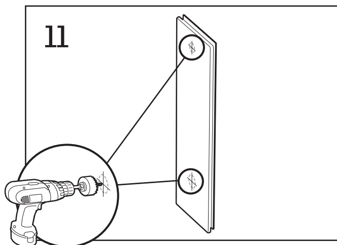
Using a hole saw (fine tooth or abrasive grit cutting edge), make necessary openings for filler and valves, drilling from inside (smooth side) out.
