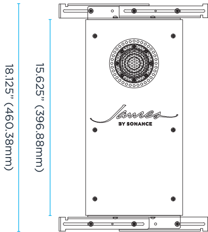
7.75" (196.85mm) Enclosure + Bracket Front View
