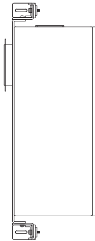
6.375" (161.93mm) Enclosure Depth Side View
