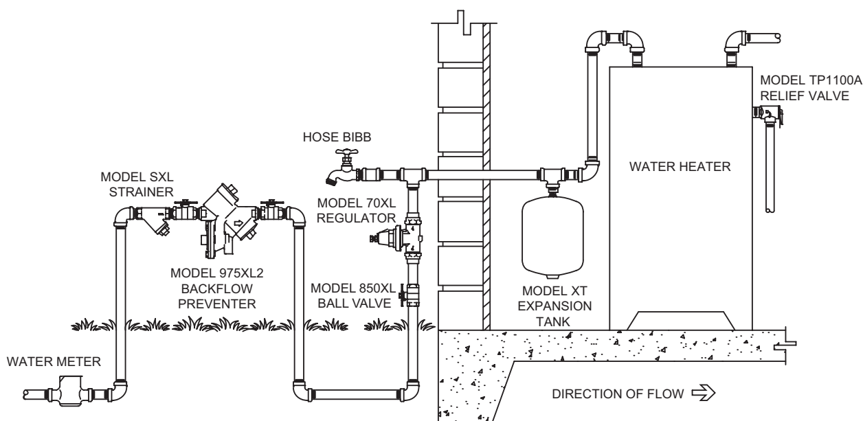
Typical Installation
