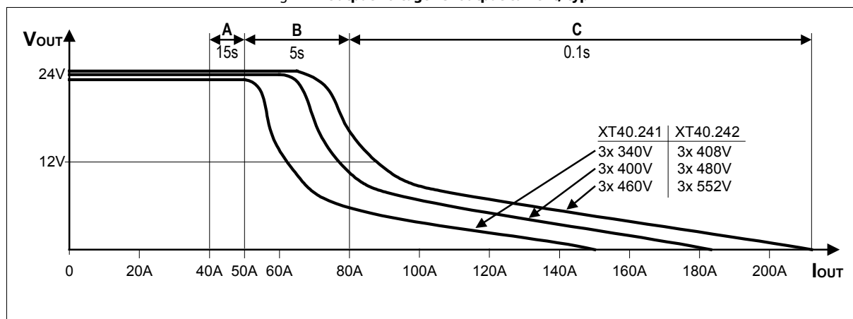
Fig. 7-1 Output voltage vs. output current, typ.
