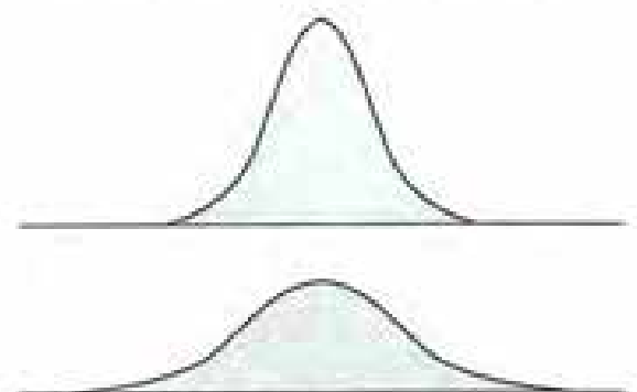
Figure 1.8. Gaussian distributions: narrow, with smaller s (top), and wide, with larger s (bottom).
