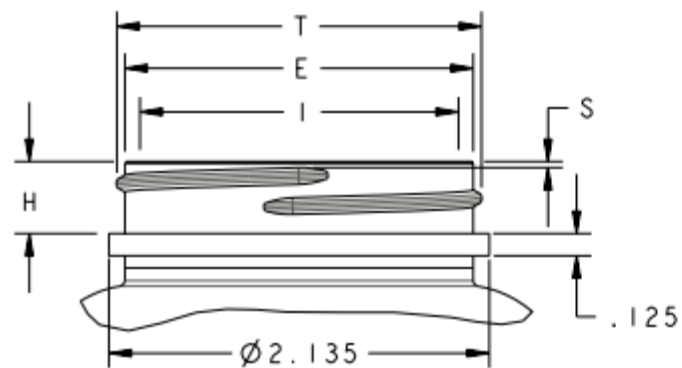
DETAIL A SCALE 3/2
