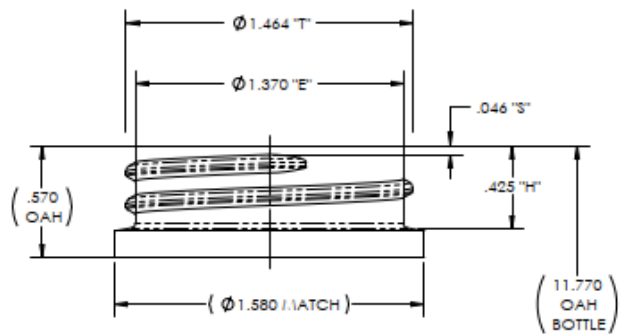
38mm SP-400 NECK FINISH DETAIL 2X SCALE
