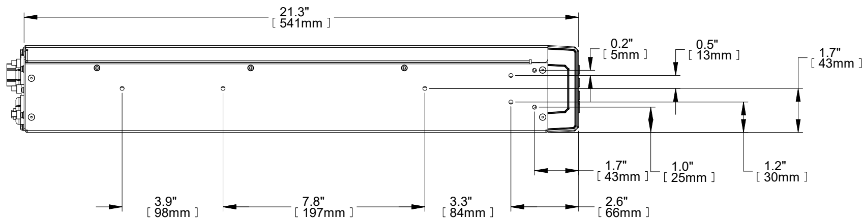
SIDE VIEW
