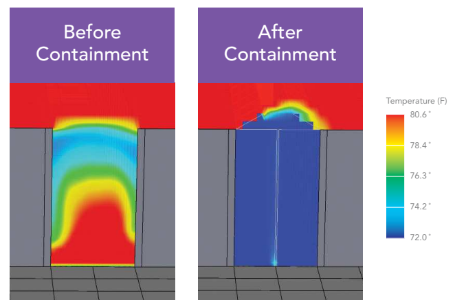
CFD analysis shows a significant reduction in hot air recirculation when Sliding Doors are applied in conjunction with Rack Top Baffles at the end of the cold aisle.
