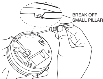
Figure 7a - How to Tamperproof
