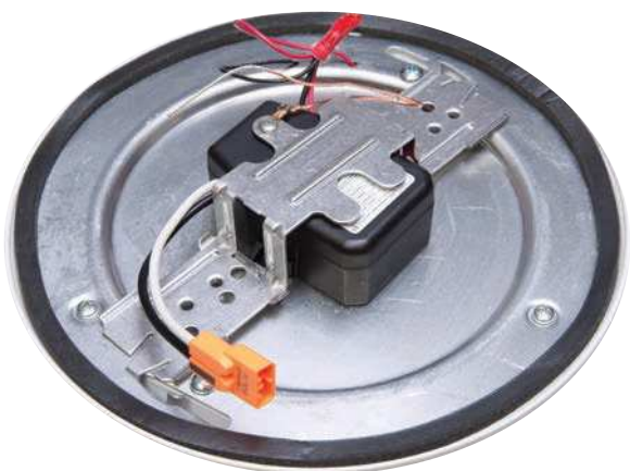
SLD6 with junction box bracket installed.
