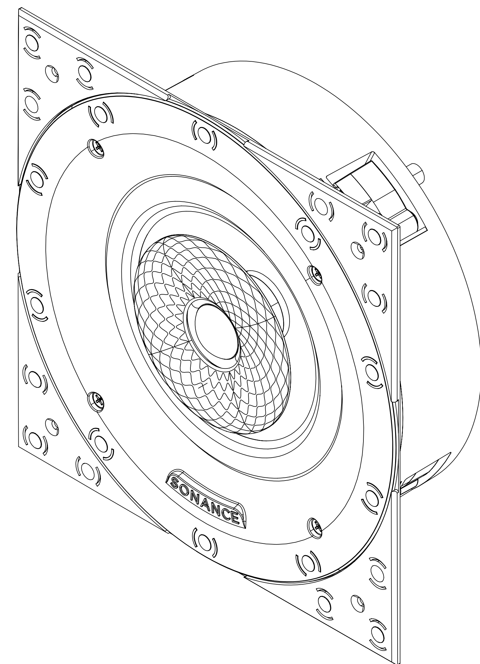
ISOMETRIC
