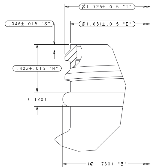
FINISH DETAIL SCALE 5:1
