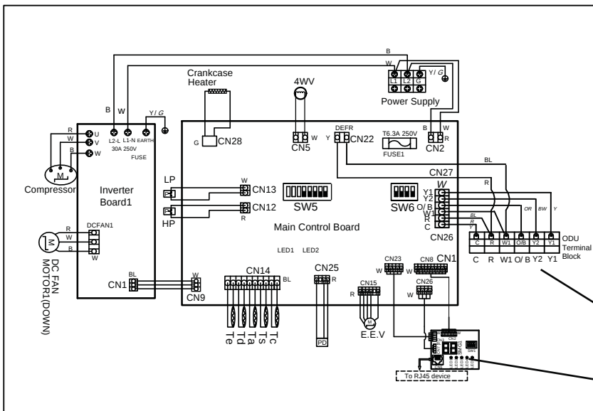
Figure 20. 60K Wiring Diagram
