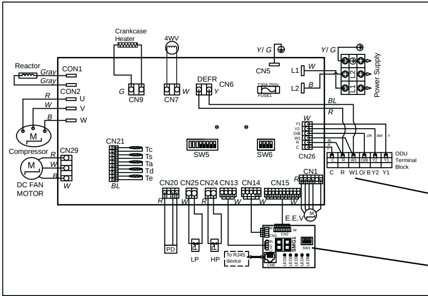
Figure 19. 18K/24K/30K/36K/42K/48K Wiring Diagram
