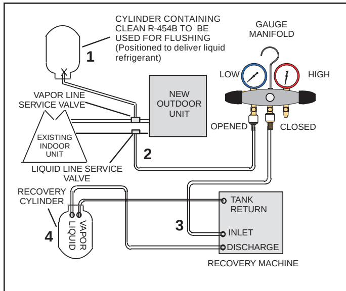
Figure 15. Connecting Gauges
