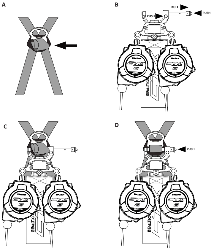
Figure 5 - CT-X Cable Class 2 Leading Edge SRL-P Installation
