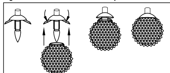
Figure #4--Ball Shade assembly.
