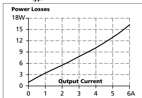
Fig. 7-2 Losses vs. output current at 24V, typ.
