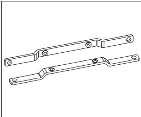
Fig. 22-1 ZM1.WALL Wall mounting bracket
