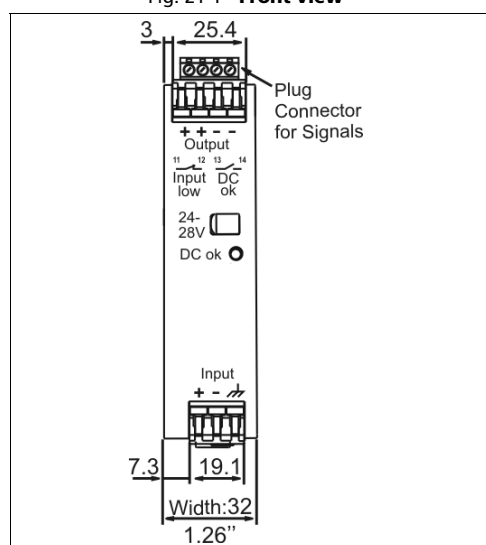
Fig. 21-1 Front view
