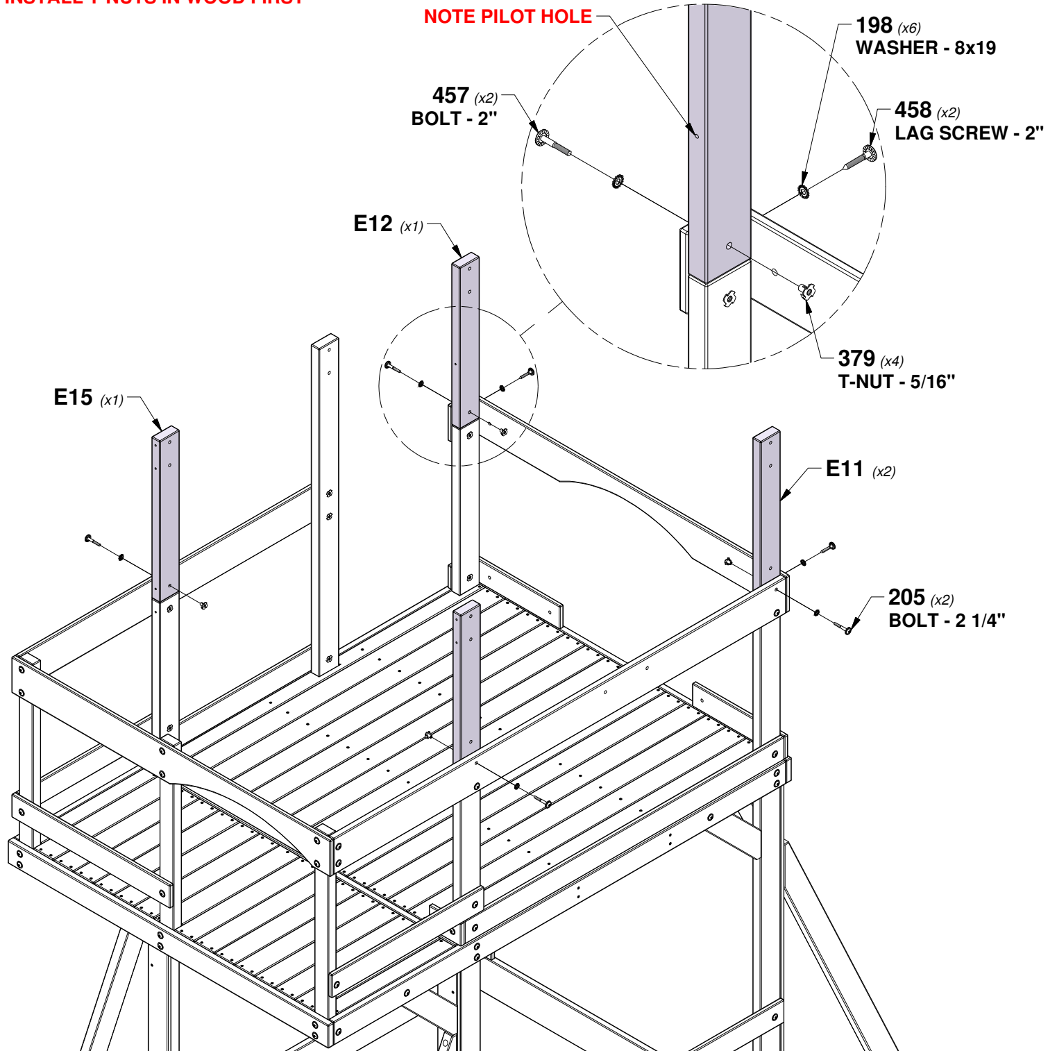
E15 | FORT UPRIGHT - W4L16593 (x1) | 1 3/8"x3 3/8"x23 3/4" (36x86x602)
