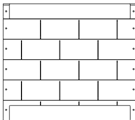
WP6 | REAR CENTER WALL - W2A03506 (x1) | 1 1/4"x18 1/4"x20 7/8" (32x465x530)
