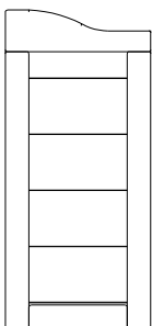
DP1 | RIGHT DOOR ASSEMBLY - W2A01927 (x1) | 1 1/8"x8 3/8"x18 1/8" (27x211x460)
