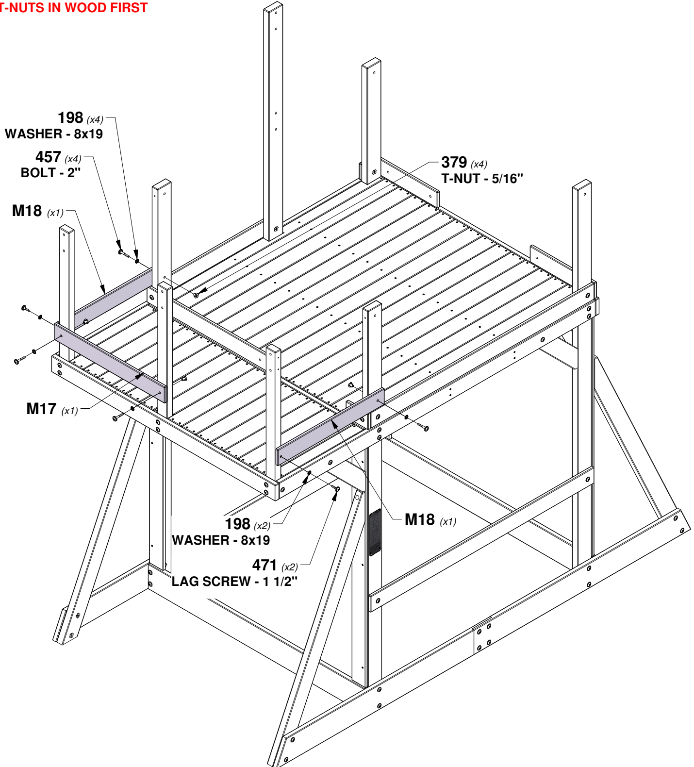
M18 | WALL RAIL - W4L06461 (x2) 5/8"x3 3/8"x25 7/8" (16x86x658)
