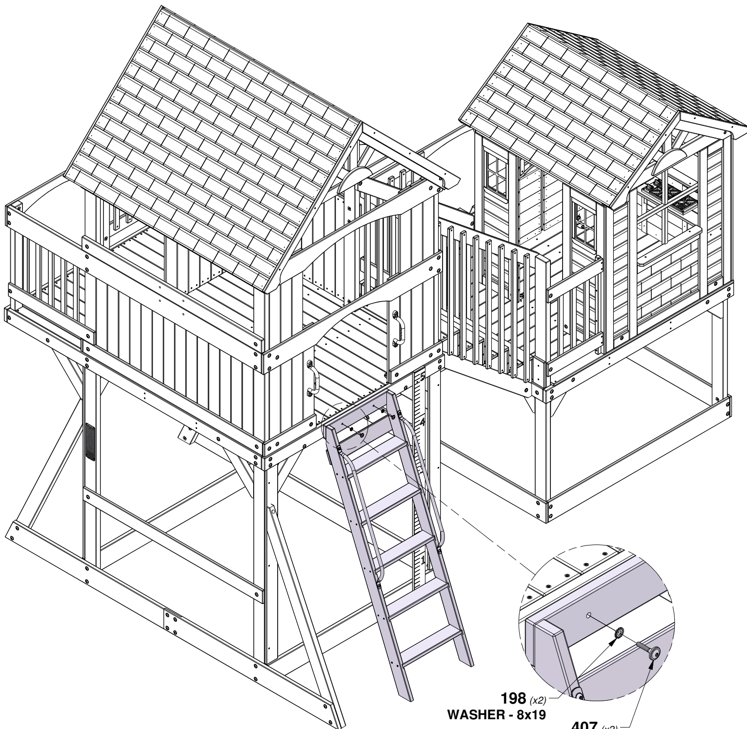
5 FT. LADDER ASSEMBLY
