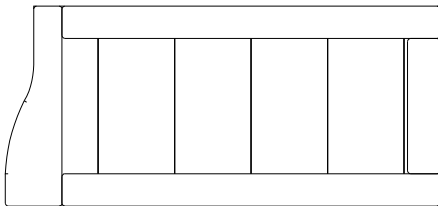
DP1 | RIGHT DOOR ASSEMBLY - W2A01927 (x1) | 1 1/8"x8 3/8"x18 1/8" (27x211x460)
