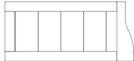
DP2 | LEFT DOOR ASSEMBLY - W2A01928 (x1) | 1 1/8"x8 3/8"x18 1/8" (27x211x460)
