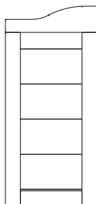
DP2 | LEFT DOOR ASSEMBLY - W2A01928 (x1) | 1 1/8"x8 3/8"x18 1/8" (27x211x460)
