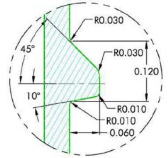
GLASS THREAD DETAIL SCALE 10 : 1
