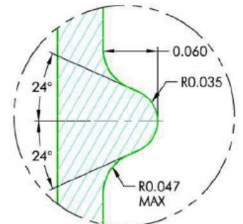
GLASS THREAD DETAIL SCALE 10 : 1
