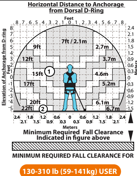
Figure 11 - FT-X Minimum Required Fall Clearance for 130 to 310 lbs. (59 to 141 kg) Users
