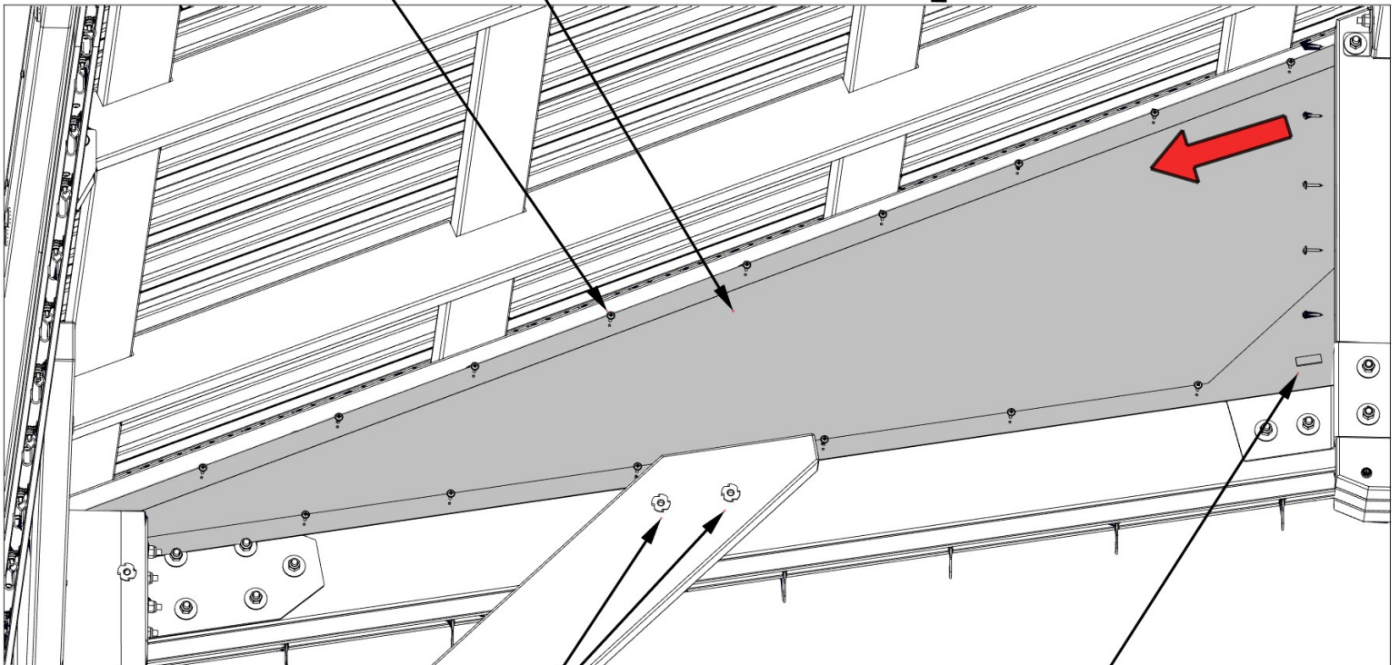
392 (x88) SCREW - 3/4"
