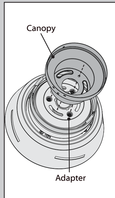
Place the canopy on the top housing. Ensure all four screw holes line up with the screw holes in both the top housing and the adapter.
