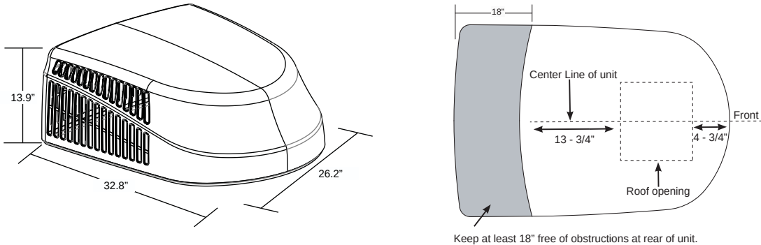
Figure 1: Standard Height Rooftop Unit (GRCS/GRHS):
