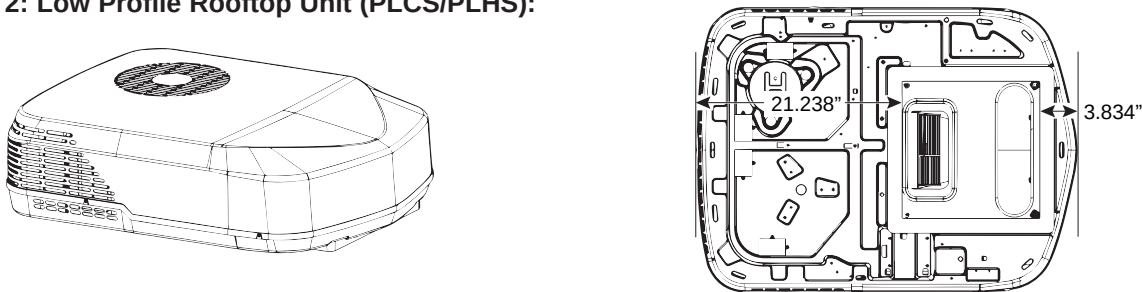
Figure 2: Low Profile Rooftop Unit (PLCS/PLHS):
