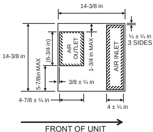
Standard Height Models (GRCS/GRHS) TOP-DOWN VIEW
