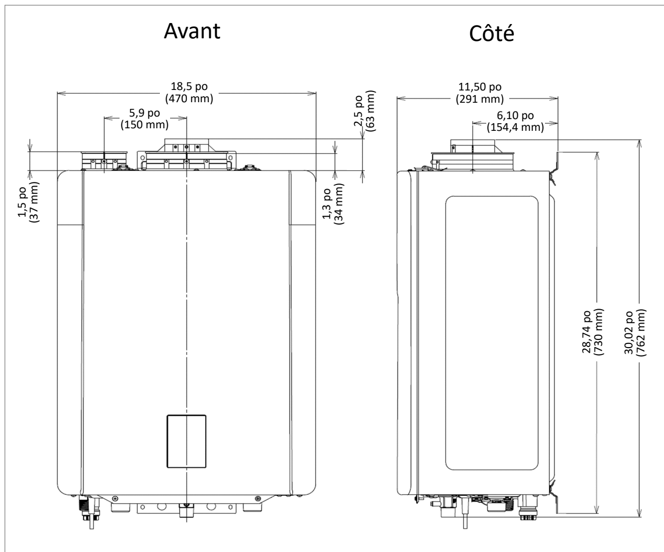
Figure 5: Dimensions
