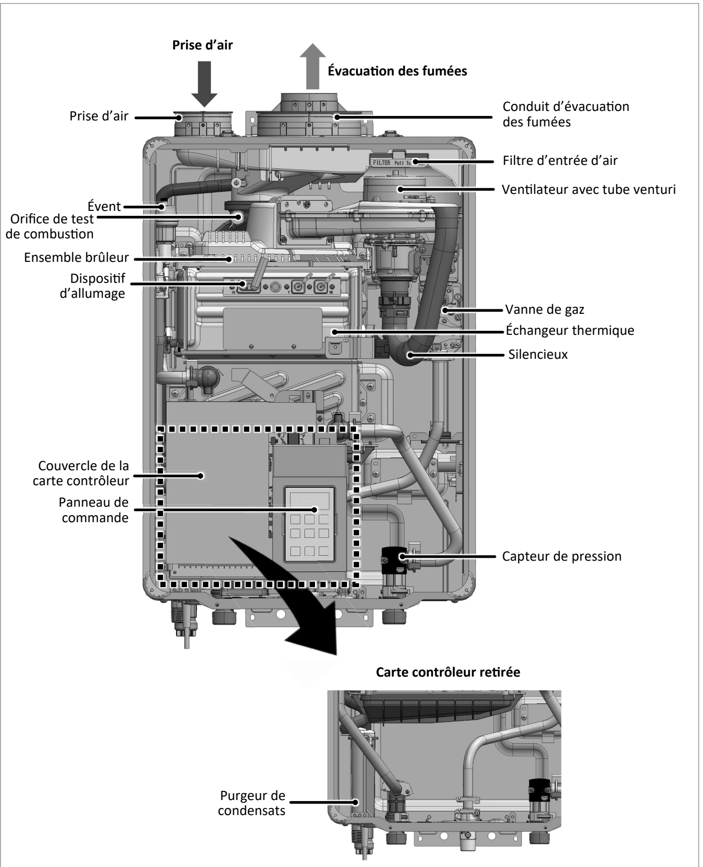
Figure 4: Composants
