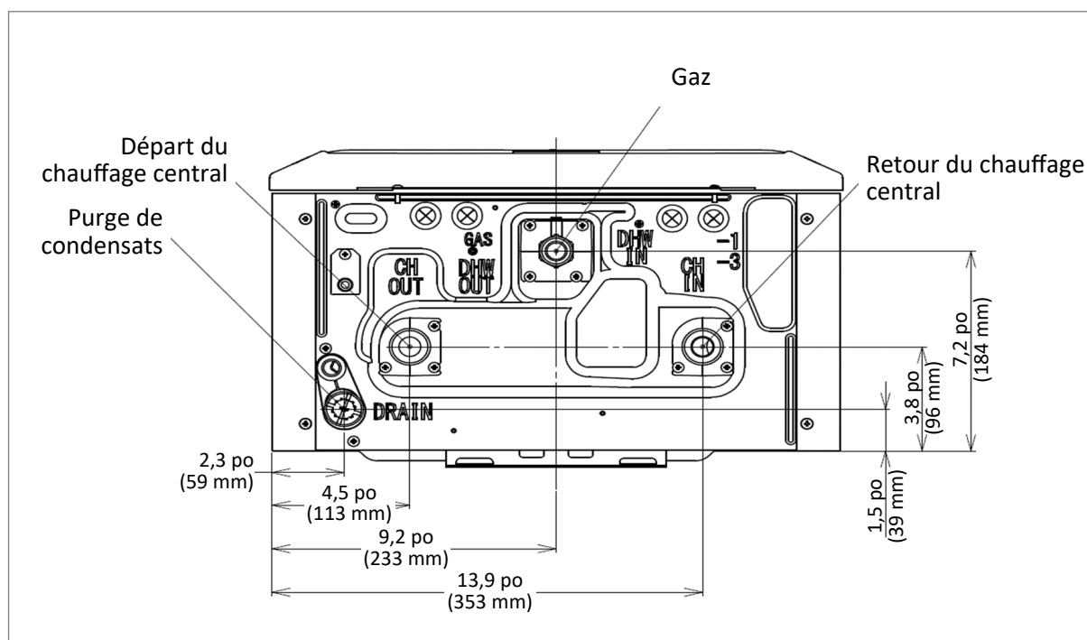
Figure 6: Raccords d'alimentation
