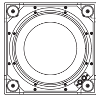
EMB10-70-M WIDTH Bottom View
