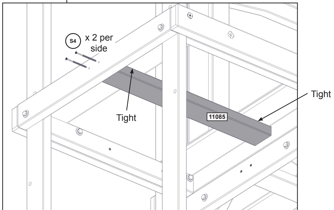
Underneath View
