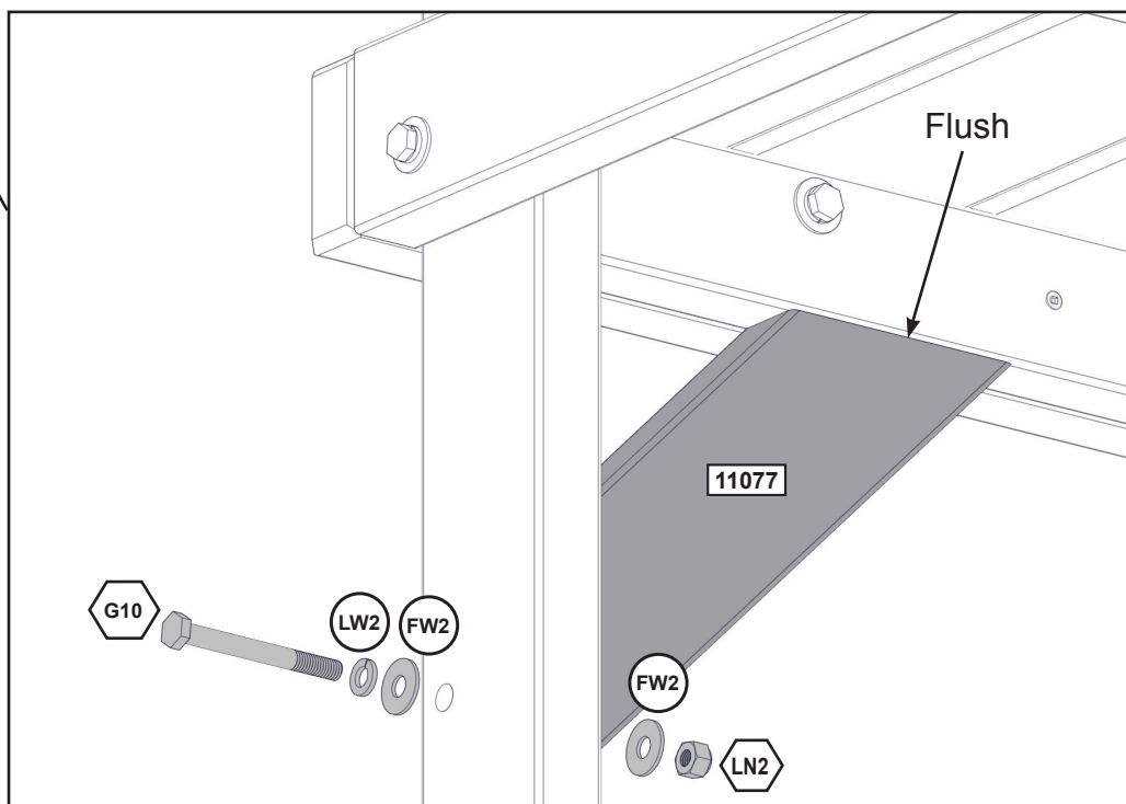
Underneath View
