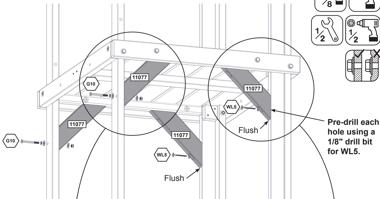
Underneath View
