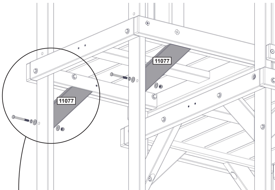
Underneath View
