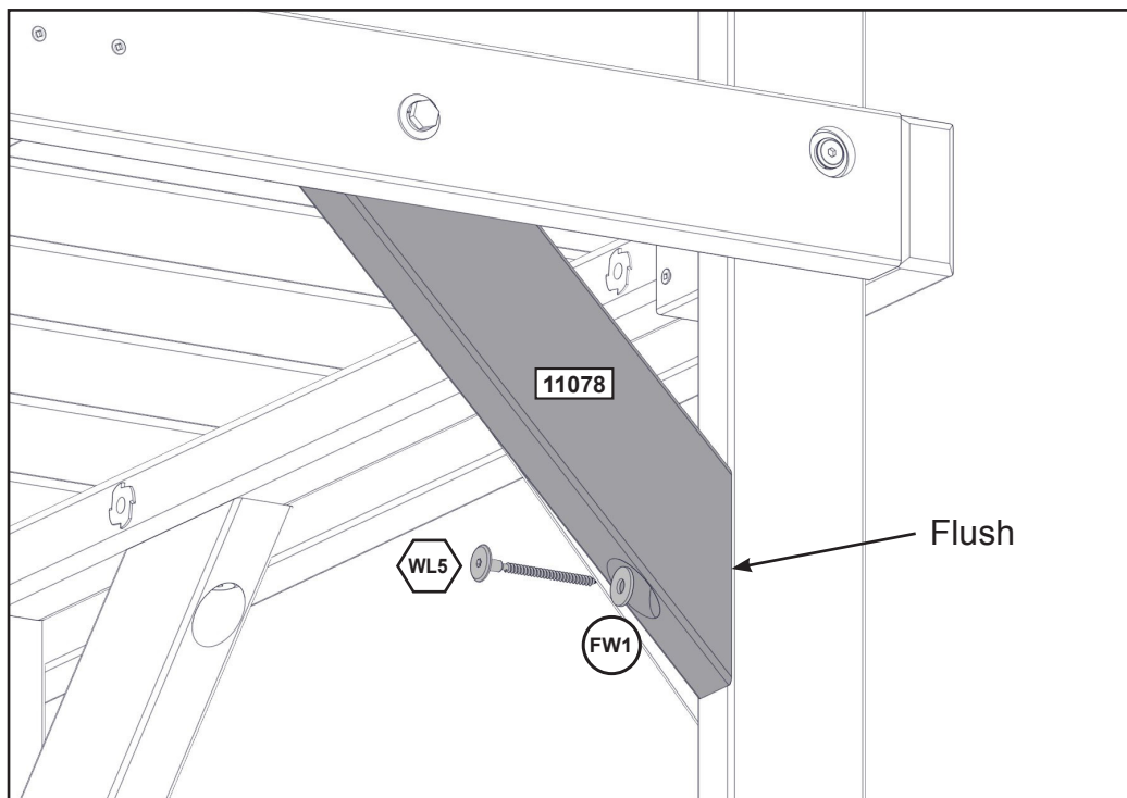
Underneath View
