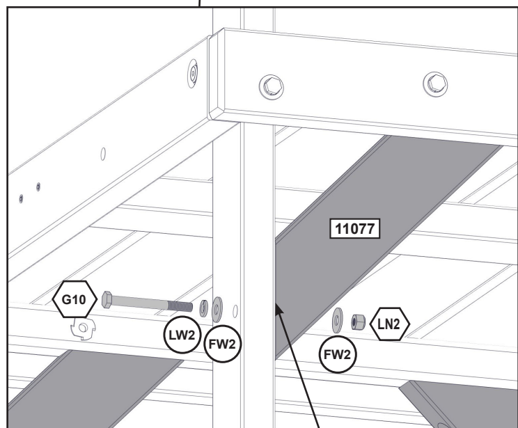
Underneath View
