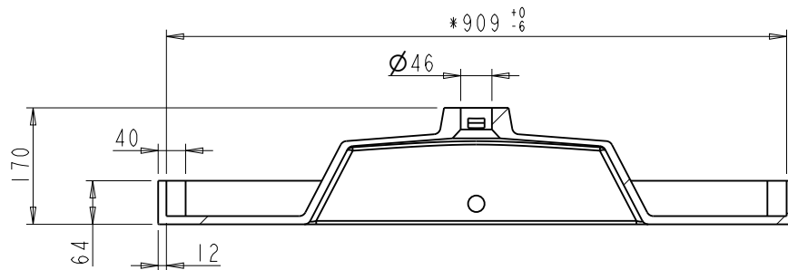
SECTION B-B
