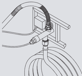
gas valve / bellows connection
