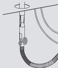
inlet tube / bellows connection
