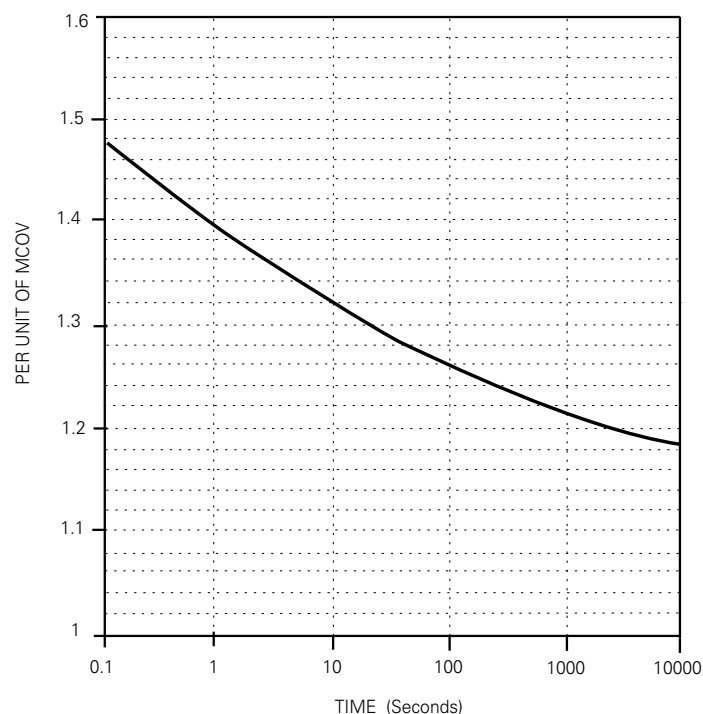
Figure 9. Storm Trapper H.E. temporary overvoltage capability
