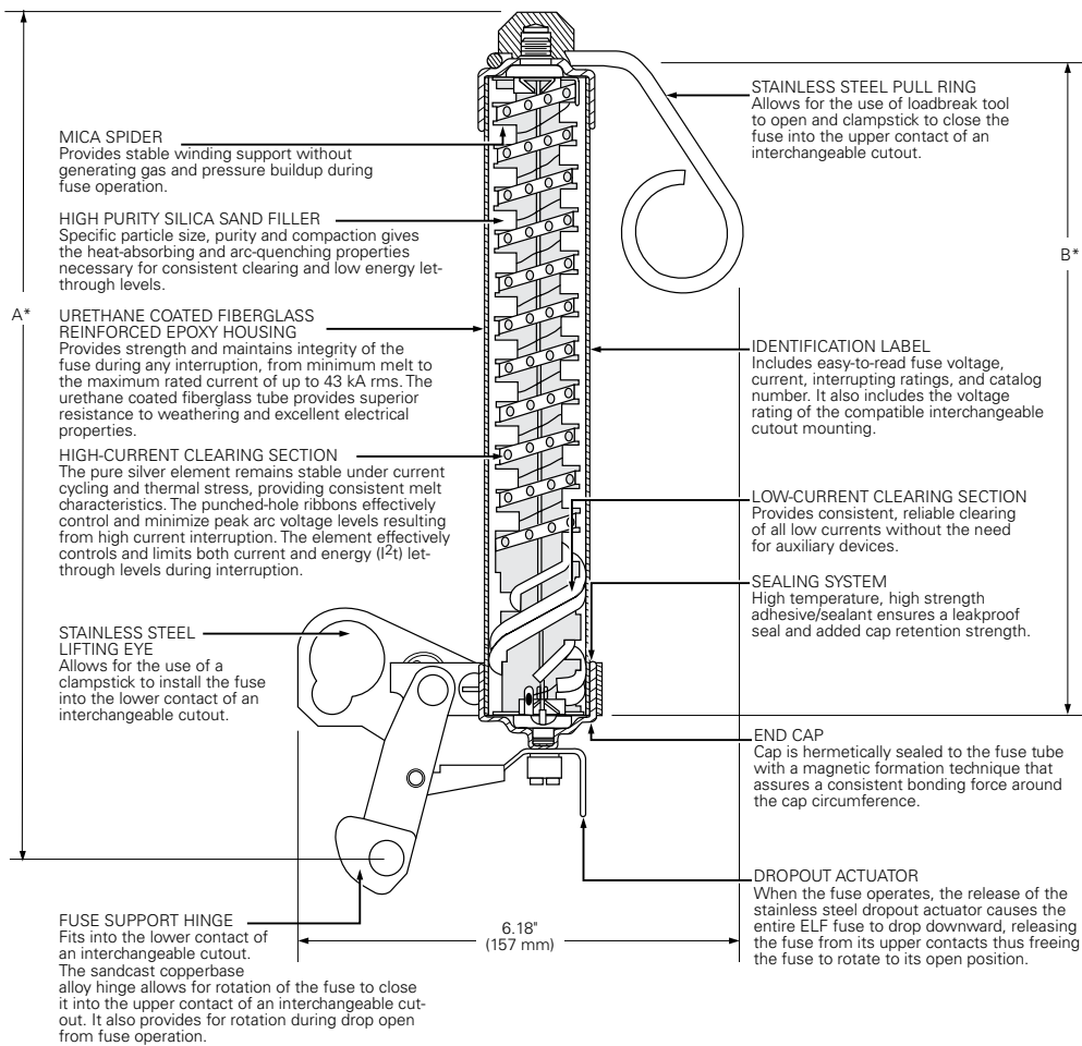
Figure 33. Double/triple barrel ELF fuse dimensions
