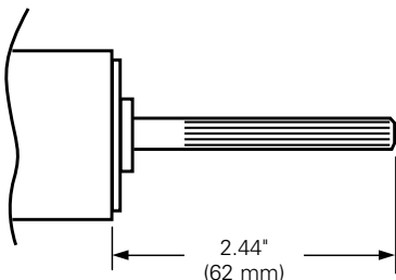
Figure 37. Spline stud terminal (-G)
