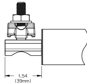
Figure 42. Medium parallel-groove terminal (#8-2/0 cable sizes) (-P)
