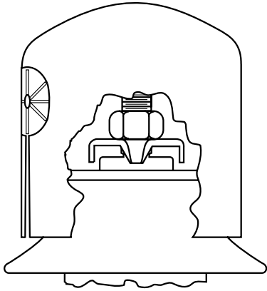
A = Silicon bronze nut, stainless steel wire clamp and universal wildlife protector.
