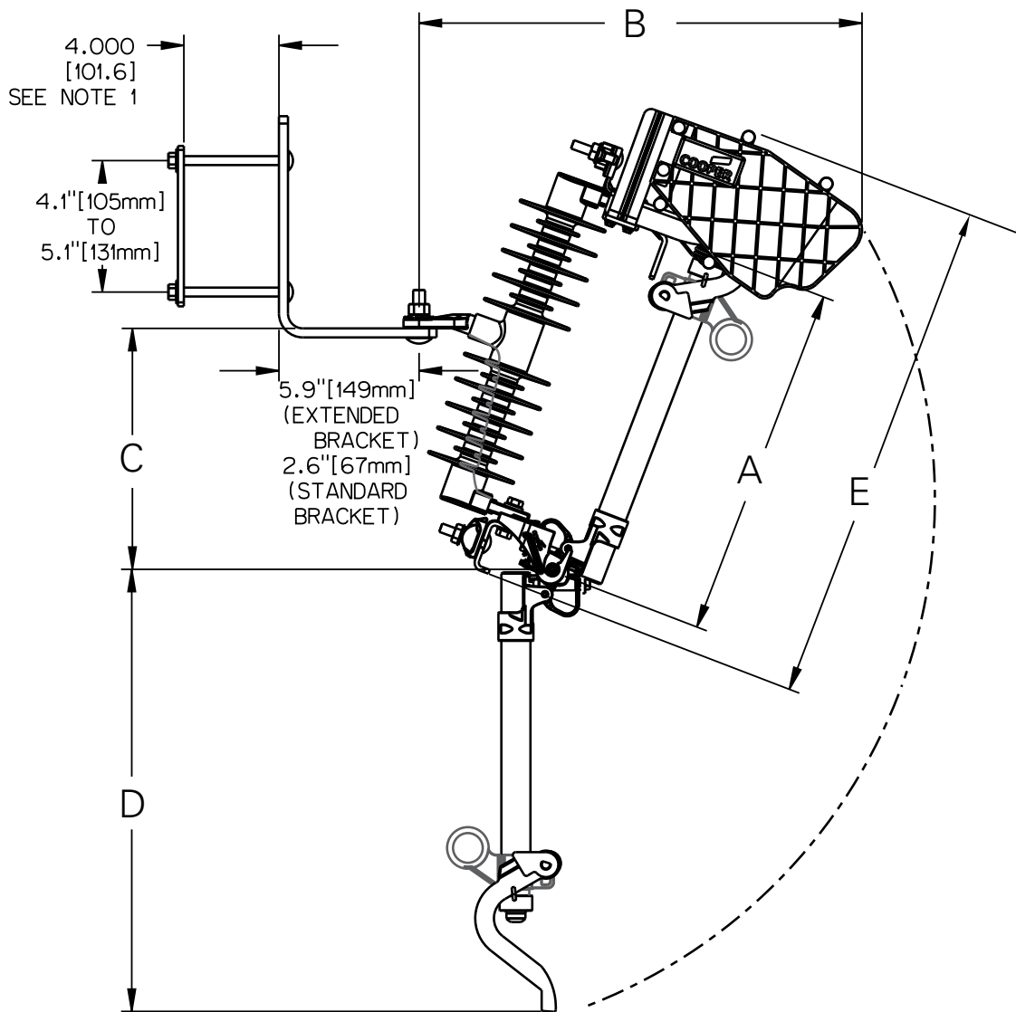
Figure 25. Loadbreak Type LB cutout assembly
