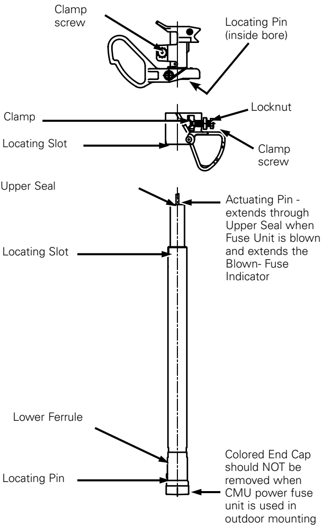
Figure 49. Outdoor CMU power fuse fittings
