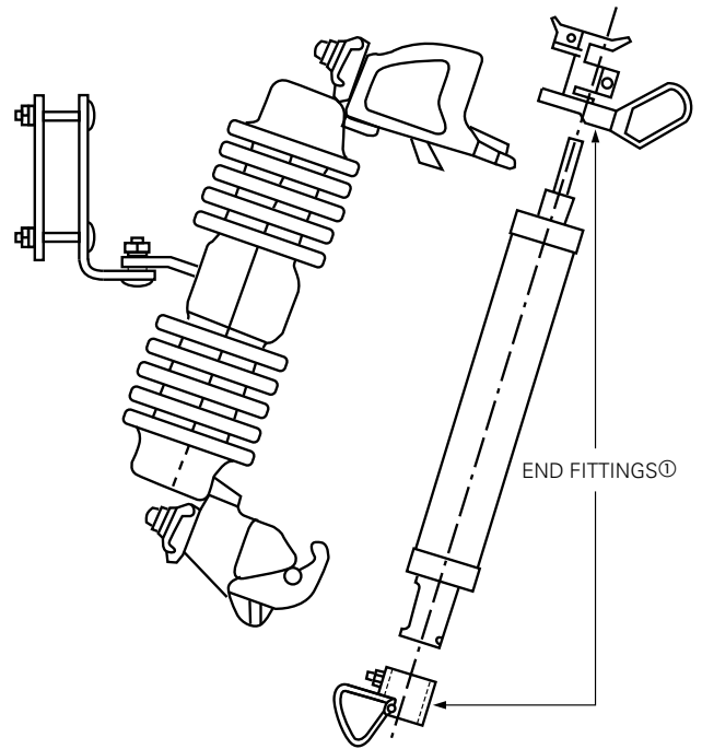
Figure 45. X-Limiter hinge-mounted fuse with dropout indication
