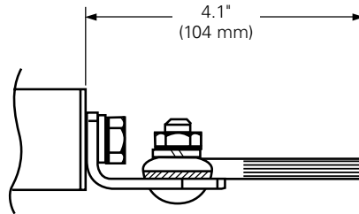
Figure 39. Universal adapter terminal (-L)
