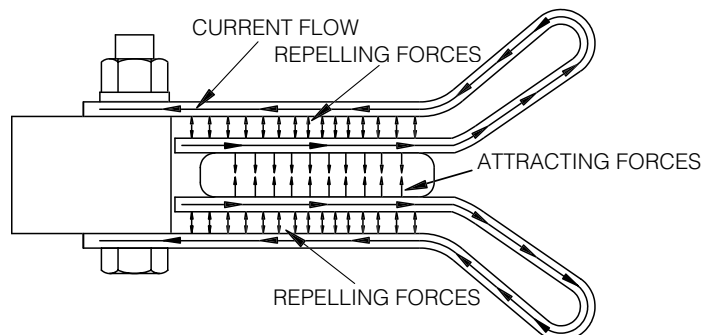
Figure 19. Magnetic forces acting on contacts
