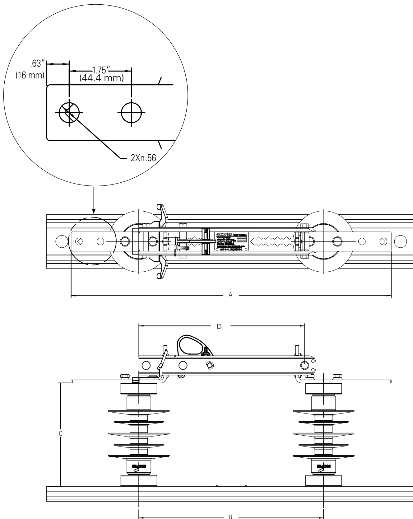
Figure 11. D-73P disconnect switch overview
