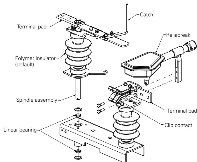
Figure 20. M-Force switch phase unit
