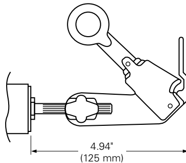
Figure 40. Hot-line clamp (-M)
