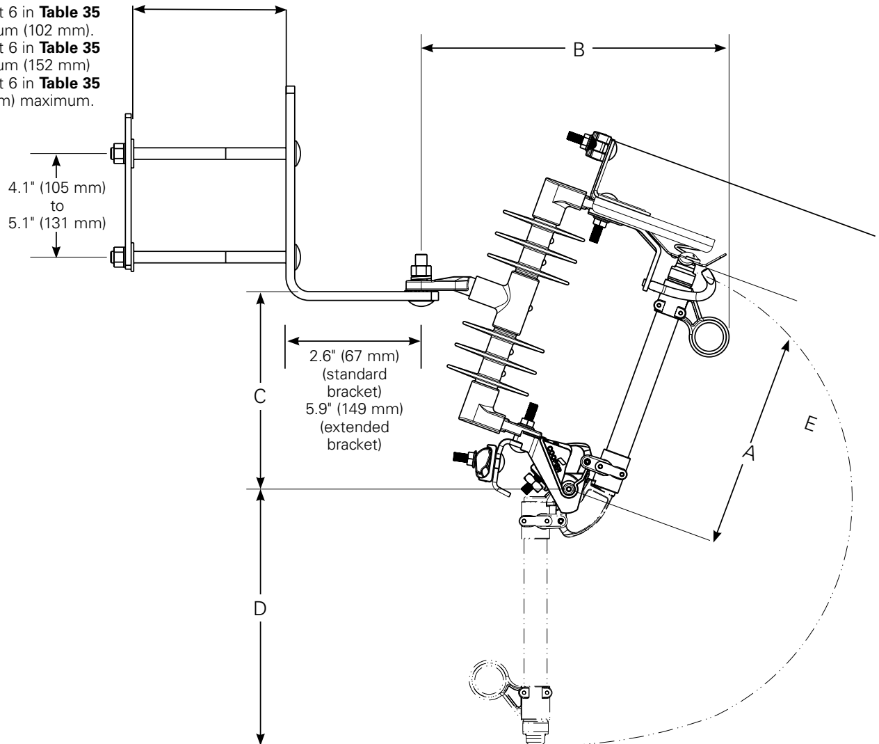
Figure 24. Polymer-insulated Type L cutout assembly
