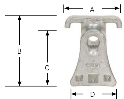
Figure 67. Iron attachments – spur
