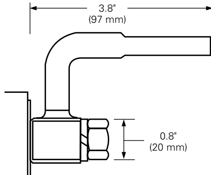
Figure 38. Offset adapter terminal (-J)
