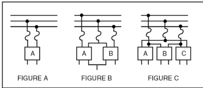
Figure 31. Schematic of primary voltage system connections
