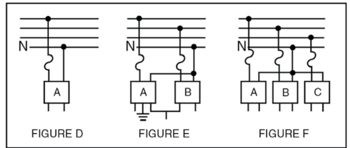
Wye-Connected Primary
