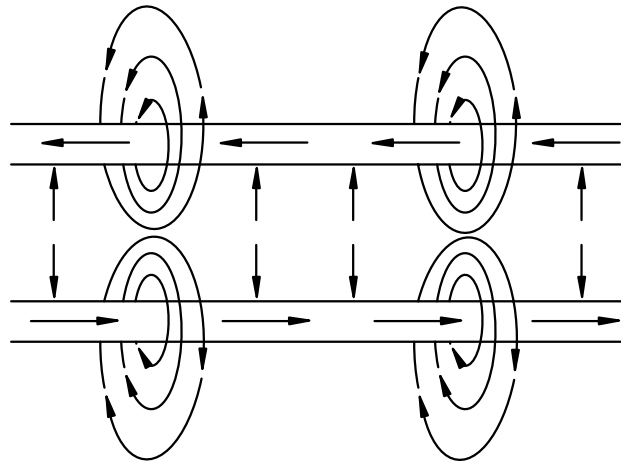
Figure 18. Current flowing in opposite direction
