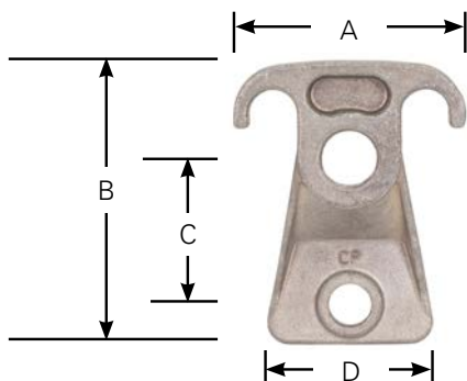
Figure 65. Aluminum attachment
