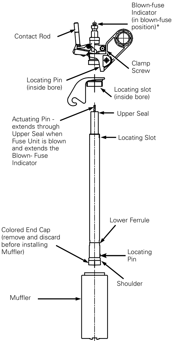
Figure 48. Indoor CMU power fuse fuse fittings
