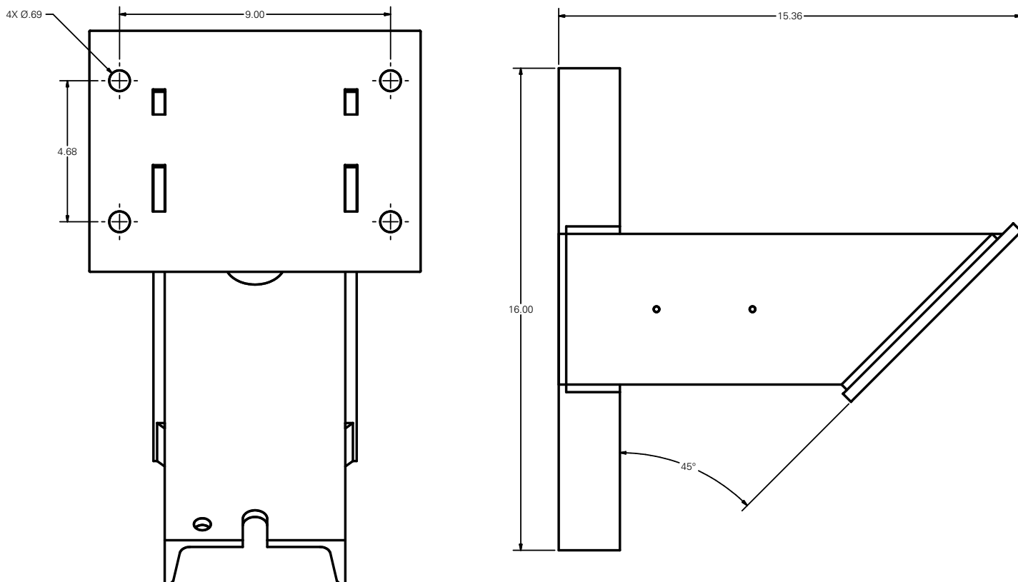
Figure 23. Pole mount bracket
