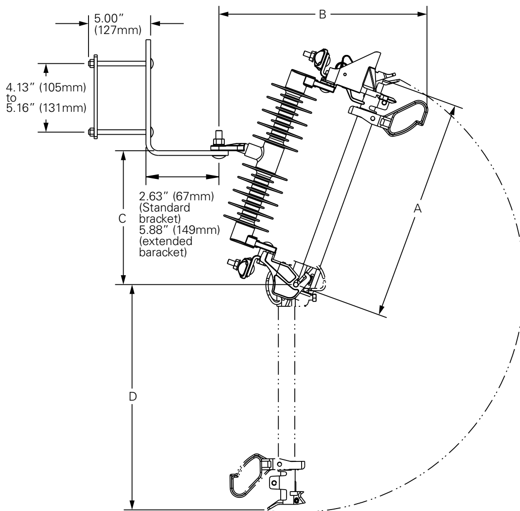
Figure 26. Eaton CMU cutout assembly
