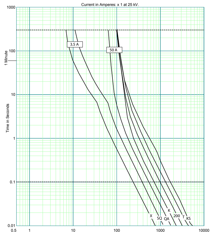
Figure 29. Kearney fuse link speed ratios
