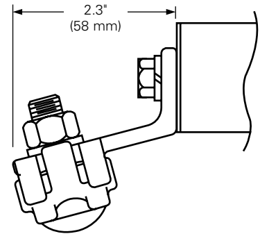
Figure 41. Large parallel-groove terminal (250 MCM) (-N)
