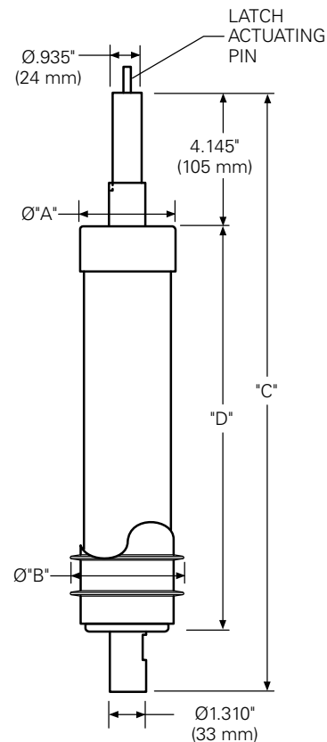
Figure 46. X-Limiter hinge-mounted fuse with dropout indication (latch actuating pin)
