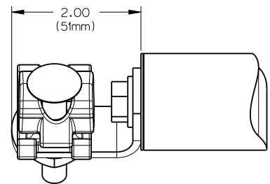
Figure 43. Parallel-groove terminal (#8-2/0 cable sizes) (-Q)
