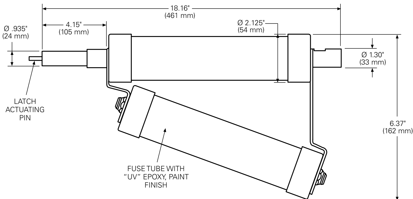
Figure 47. 17.0 kV X-Limiter hinge-mounted 65–100 A fuse with dropout indication (latch actuating pin) for Eaton's 17.0 kV CMU cutout ①
