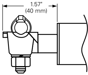
Figure 34. Eyebolt terminal (#8-2/0) (-B)
