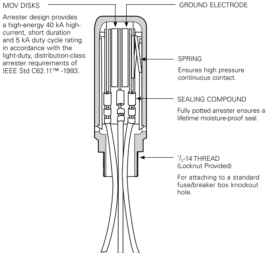
Figure 8. Cutaway of Storm Trapper H.E.
