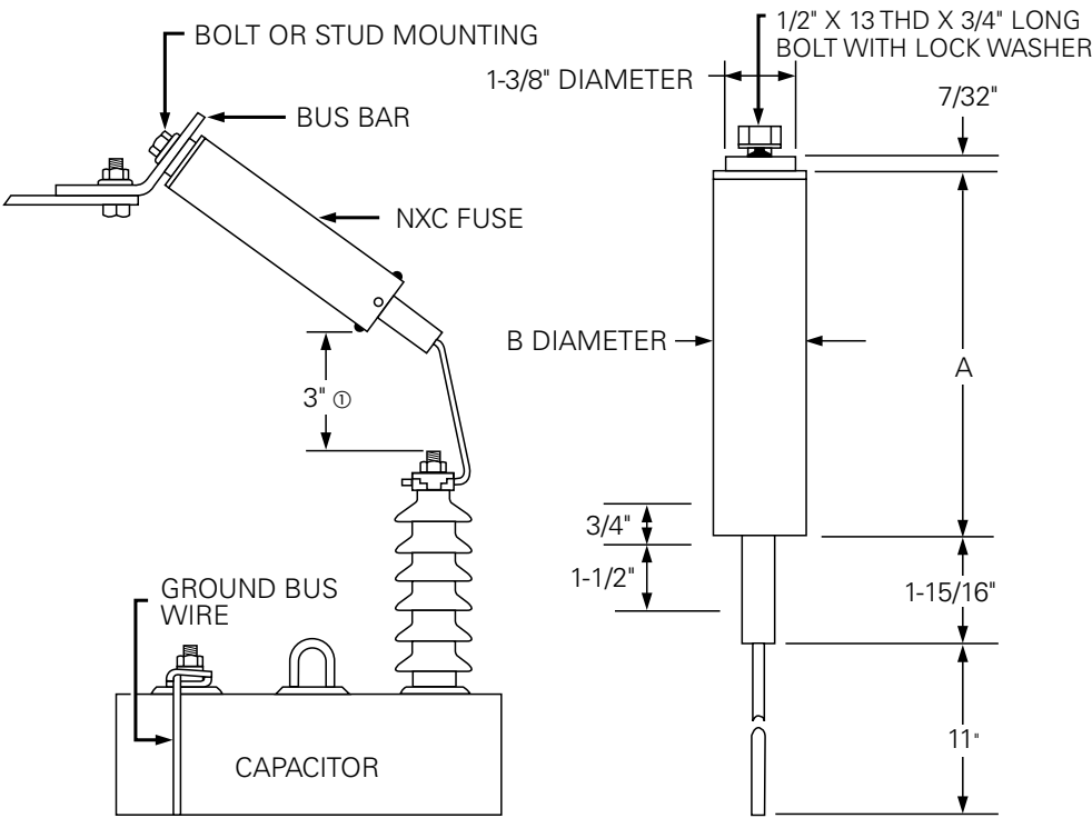
Figure 44. NXC installation
