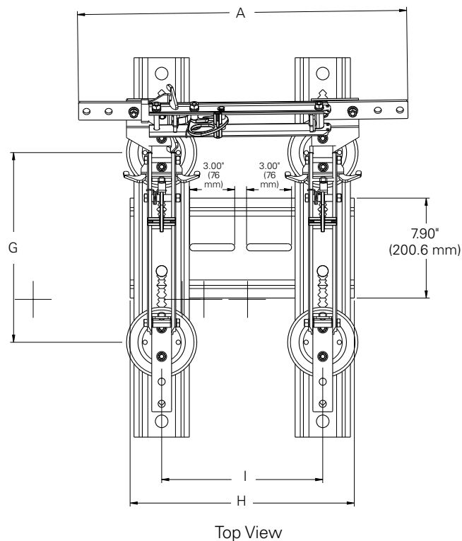
Figure 13. D-73P3 bypass switch overview
