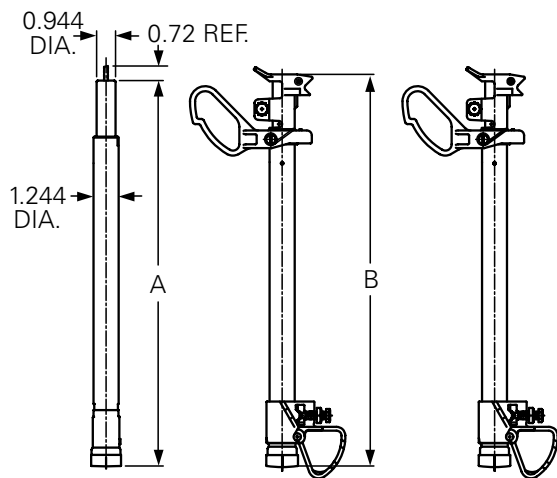
Figure 50. Outdoor CMU power fuse fitting dimensions
