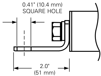
Figure 36. Spade terminal (-D)
