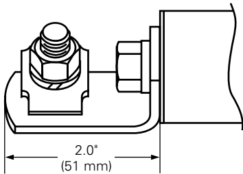
Figure 35. Parallel-groove terminal (#6-2/0) (-C)
