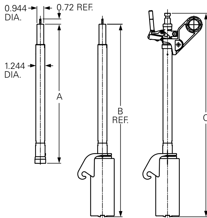
Figure 51. Outdoor (top) and indoor (bottom) dimensions
