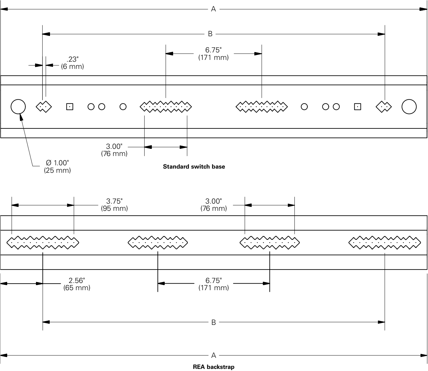
Figure 12. D-73P Disconnect switch base and backstrap options; for more options, consult catalog
