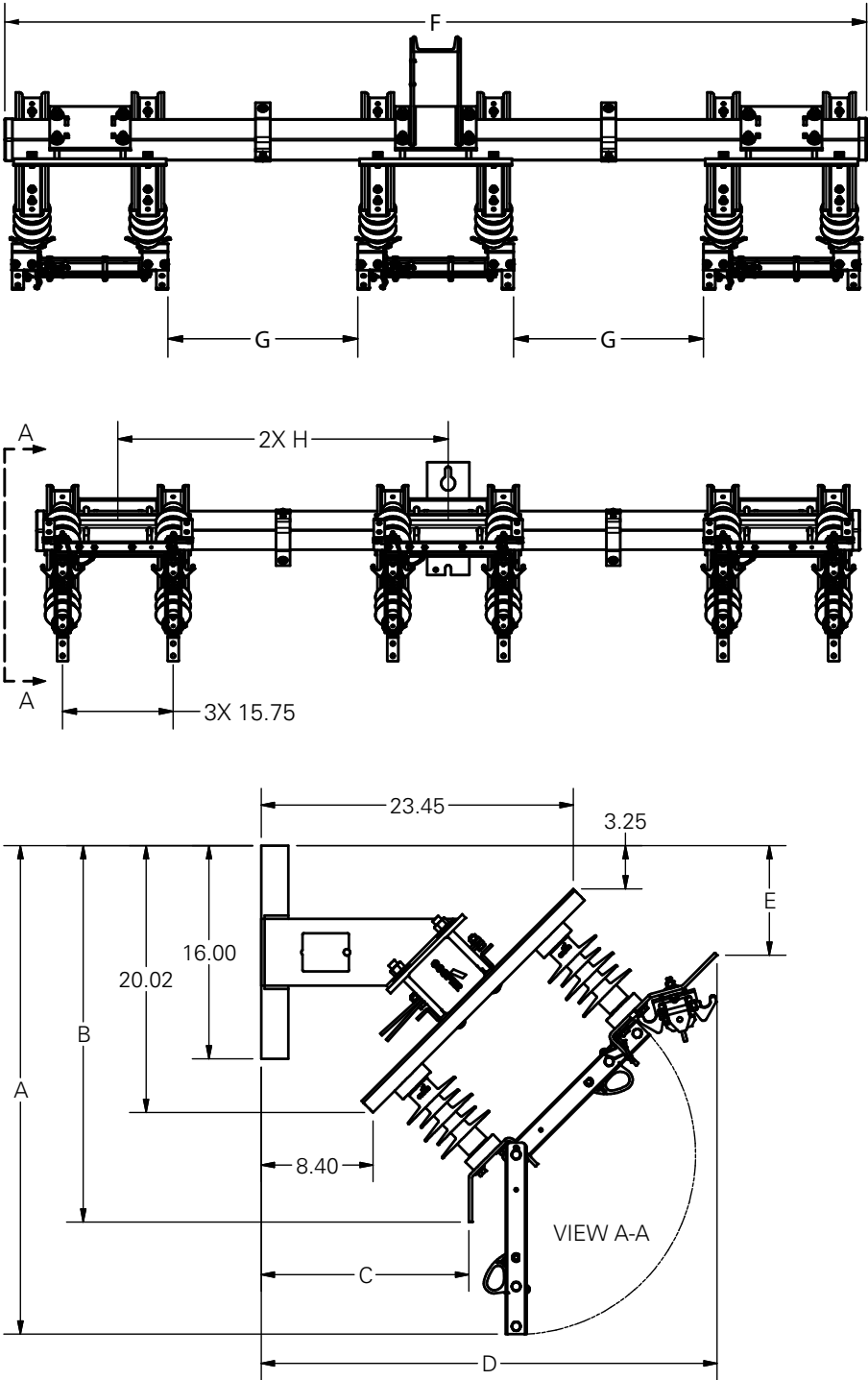
Figure 22. Top, front and side views of 3D-73P
