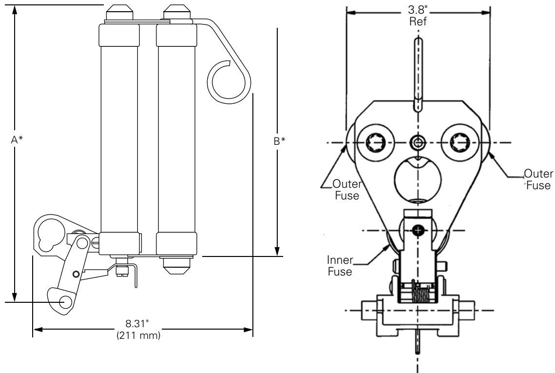
Figure 32. Double/triple barrel ELF fuse dimensions
