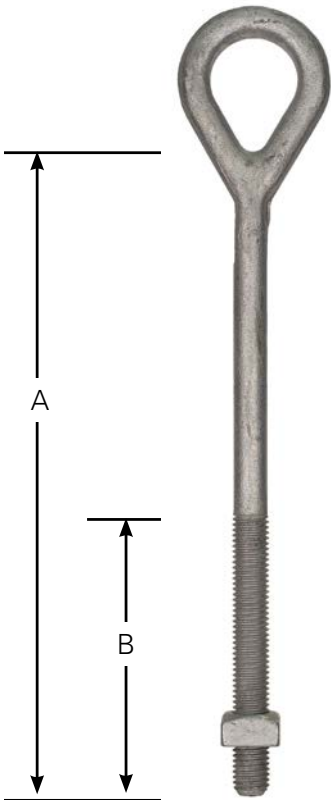
Figure 55. Ovaley eye bolt
