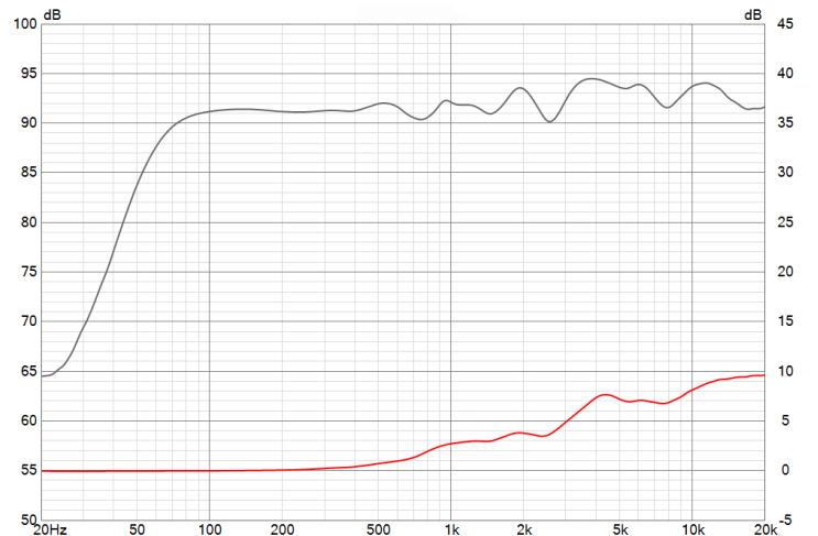
HORN SPL
