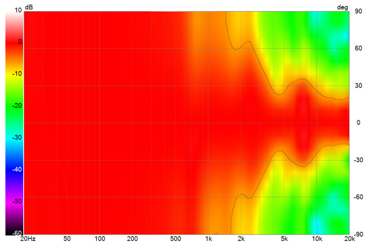
HORN DIRECTIVITY
