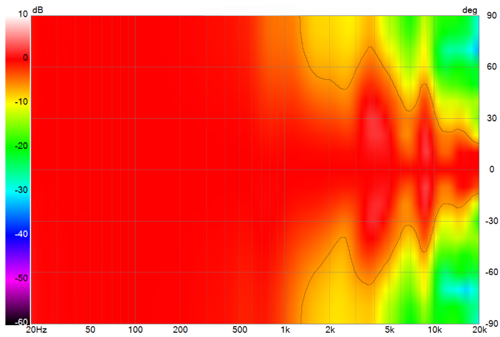
COLLAR DIRECTIVITY
