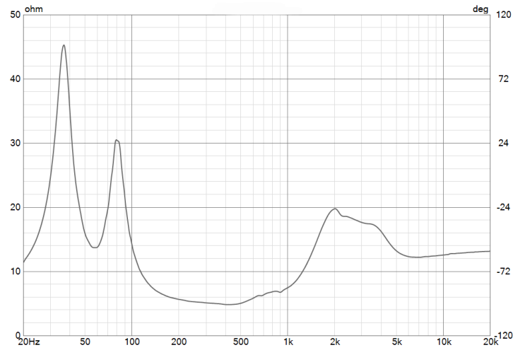
HORN IMPEDANCE
